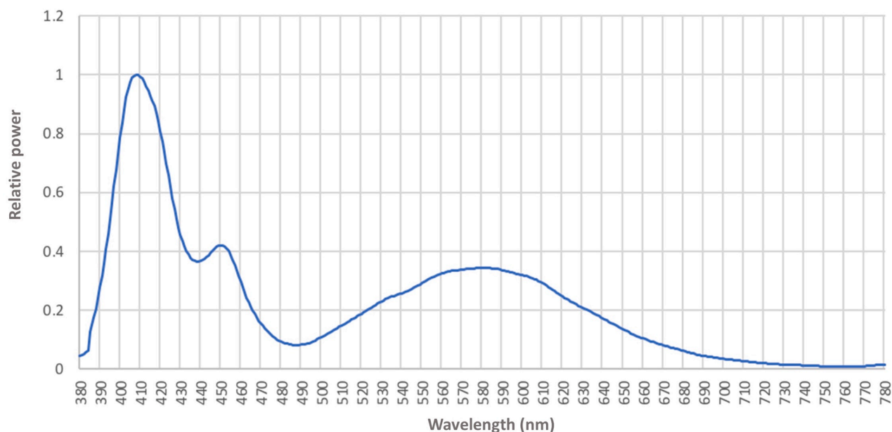
Fig. 1. A. The strip used for the experiments, consisting of 13 Biovitae® LEDs emitting wavelengths in the 400–420 nm range and delivering three different peaks within, and 37 conventional Osram Oslon (R) Square GW CSSRM2.EM-MFN2-XXX5-1 white light LEDs. The LEDs are powered at a constant current of 500 mA, guaranteed by a TCI MP 80/500 SLIM power supply. B. Relative radiometric spectral distribution of the Biovitae® strip.
